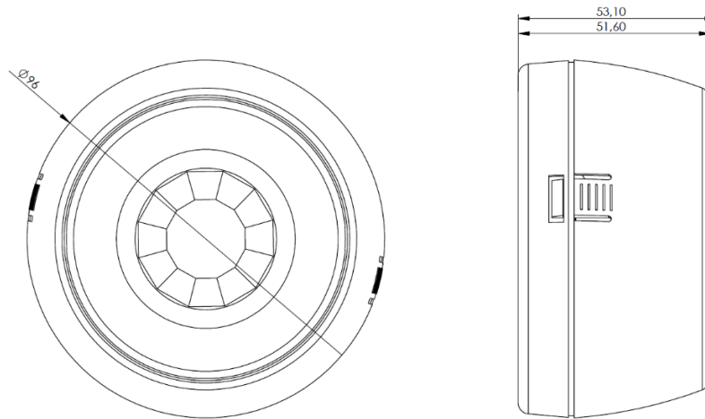
Drawing 1: XD100 Surface Mount
