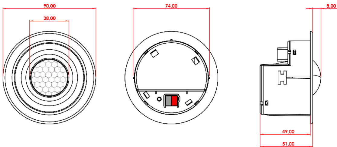
Drawing 2: XD100 Flush Mount
