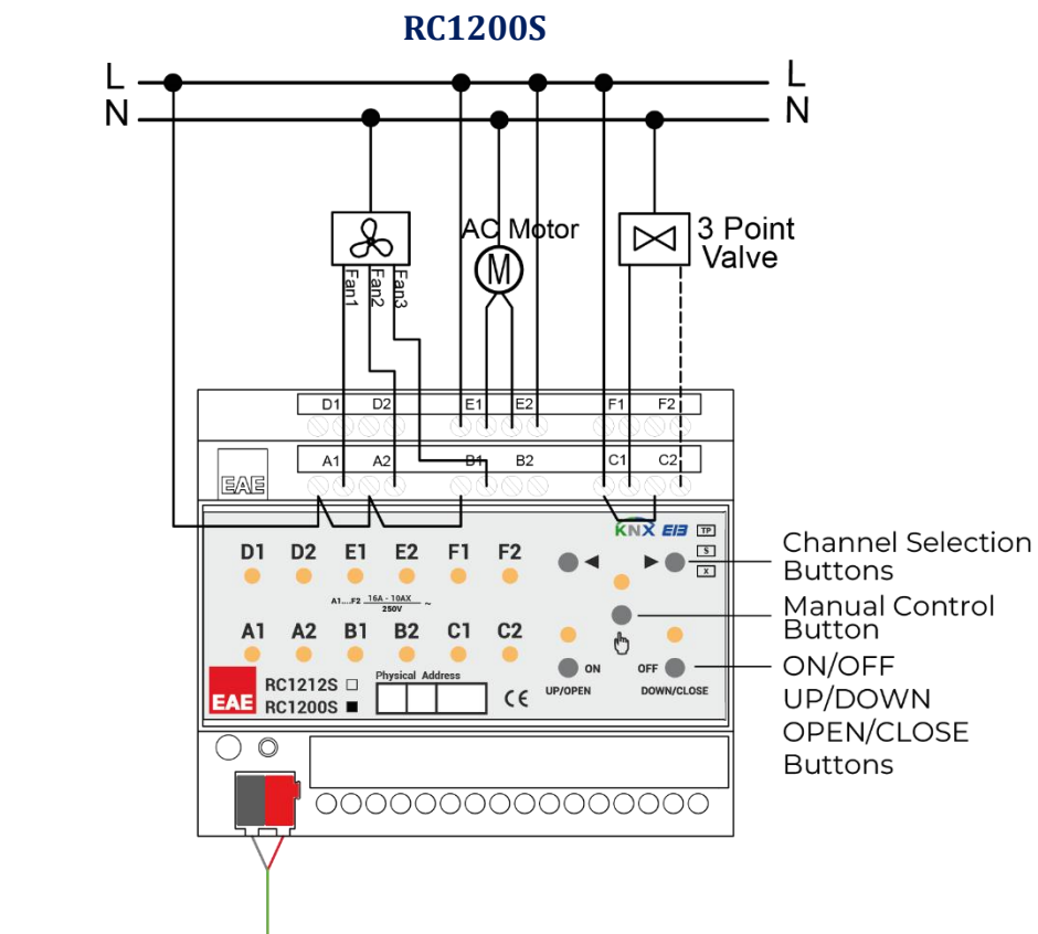
Connection Diagram 4
