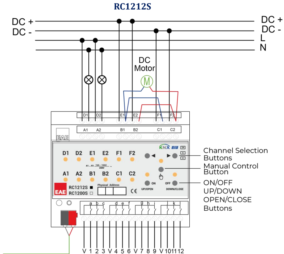
Connection Diagram 3
