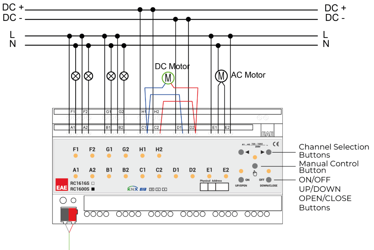
Connection Diagram 6
