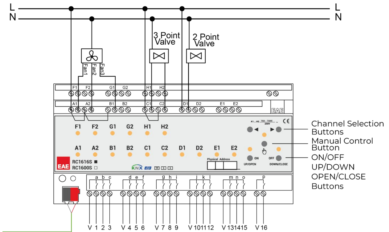
Connection Diagram 5
